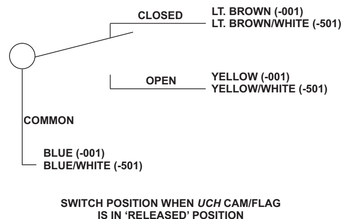
Figure 2. Microswitch in Released Position
