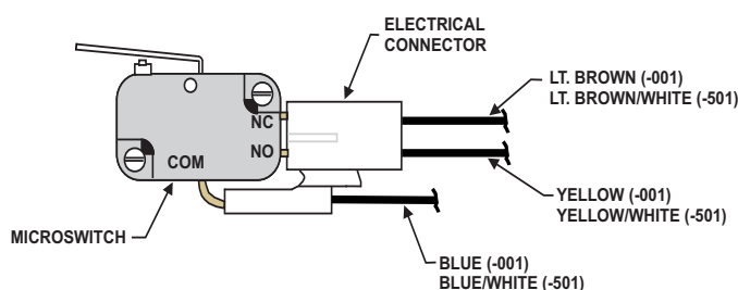
Figure 1. Quick Connect Microswitch
