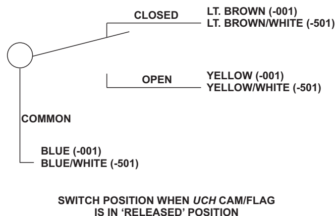
Figure 2. Microswitch in Released Position
