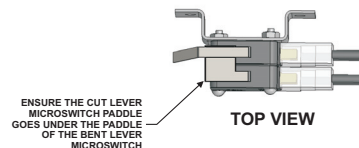
Figure 2. Dual SPDT Microswitch Kit, P/N 60-9197228-000
