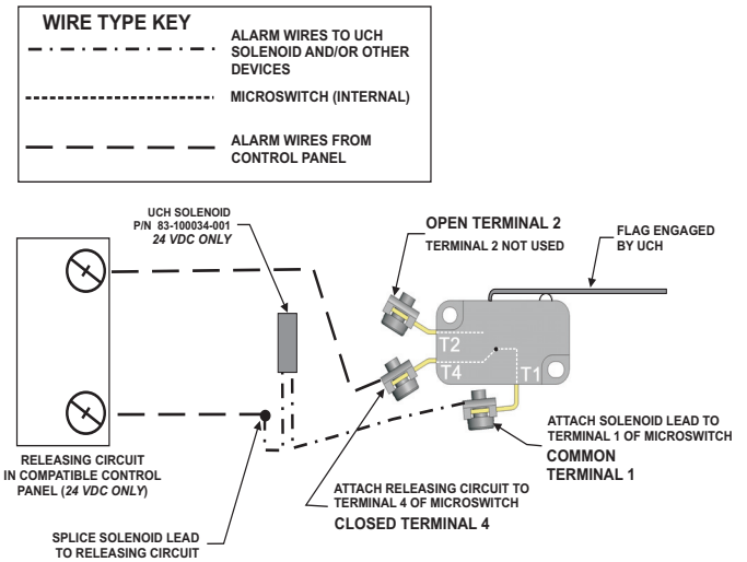
Figure 7. Release Wiring with Terminal Type Microswitch
